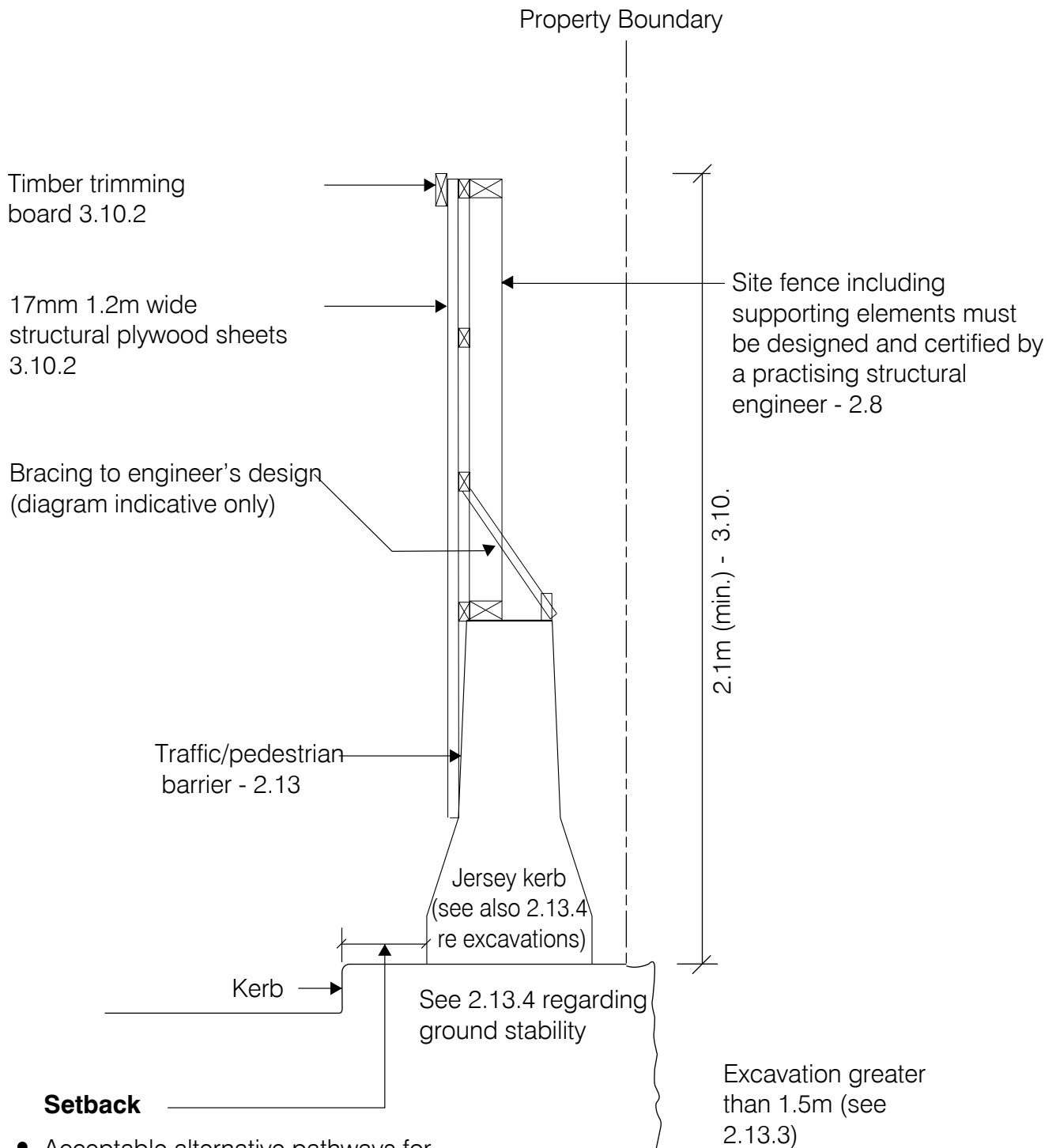
Figure 3.35: Section detail of a Type-A hoarding integrated with a traffic barrier. This design is only permitted in circumstances of a narrow footway or laneway where vehicular access and maneuvering (swept paths) to and from garages/driveways opposite can be provided and maintained. Note: The preferred design outcome is for site fences to be positioned as shown in Figure 3.5 .
